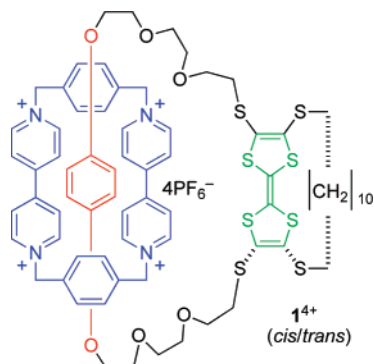
Figure 1. Molecular structure of the [2]catenane 1 \cdot 4\text{PF}_6 .
