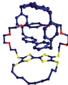
Figure 4. X-ray crystal structure of the cis isomer of the [2]catenane 1 ·4PF 6 depicted as a capped stick representation. Hydrogens, solvent molecules, and counterions are omitted for clarity.
